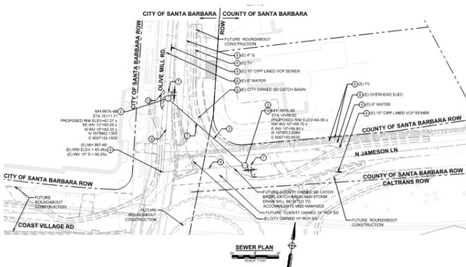
Figure 3. Roundabout Sewer Improvements North Jameson Lane and Olive Mill Road
